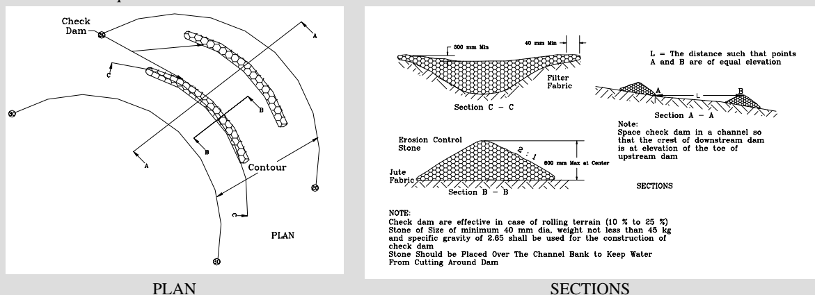
Figure 9.4: Check Dam Specification
