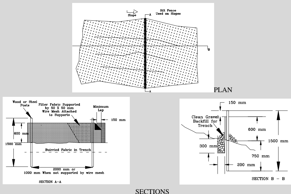
Figure 9.5 Cross-section of Silt Fencing
