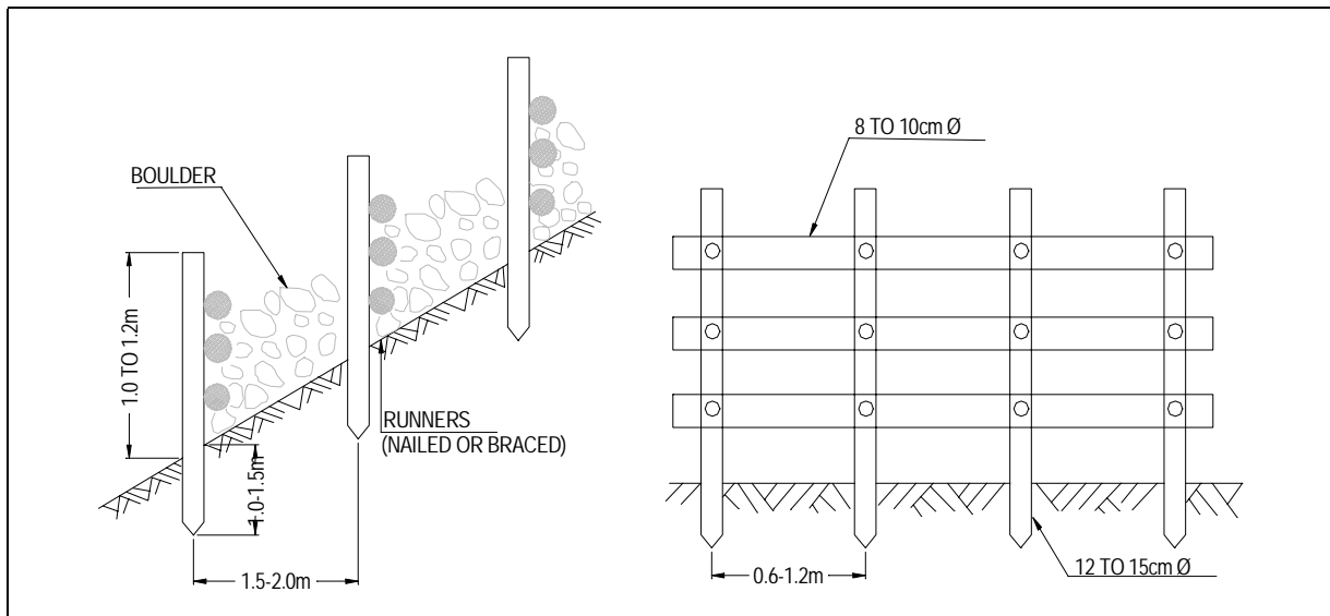
Figure 9.3: Layout and Design Specification for Bally Benching
