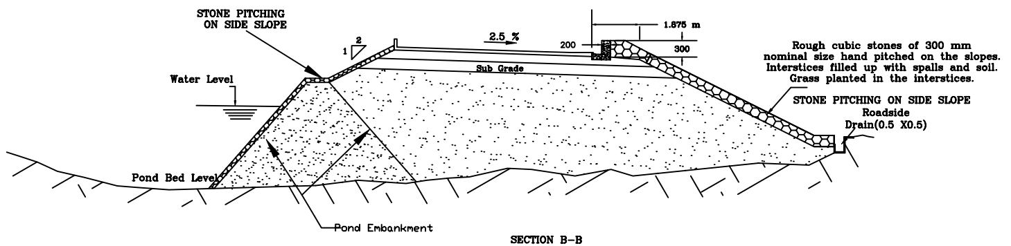
ROAD ON POND EMBANKMENT
